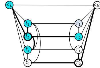
Figure 11.3: Nodes in the neighborhood of l_2 are cyan, the neighborhood of r'_2 is white. Since these neighborhoods do not intersect, the distance of these two nodes is d(l_2, r'_2) > 2 . If e.g. edge (l_2, l'_2) was included, their distance was 2.
