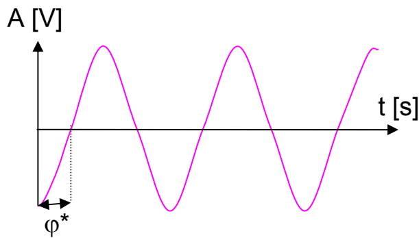
amplitude domain
