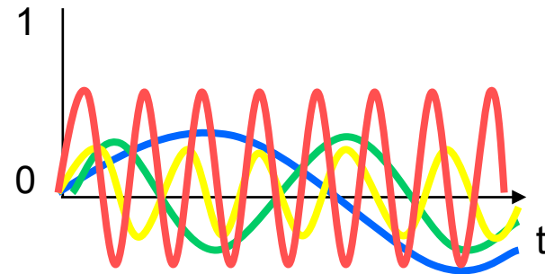
superpose harmonics
