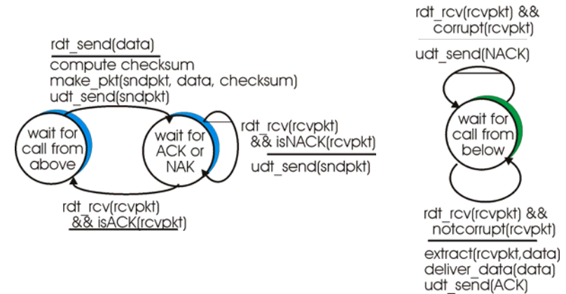
sender FSM
