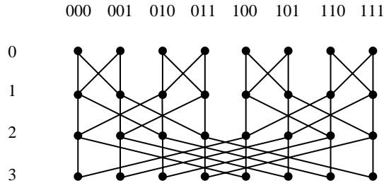
Figure 3: The structure of BF(3) .
