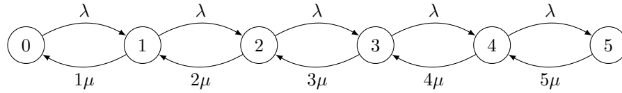
Figure 4.26: Birth-Death process modeling an M/M/5/5 queueing system.
