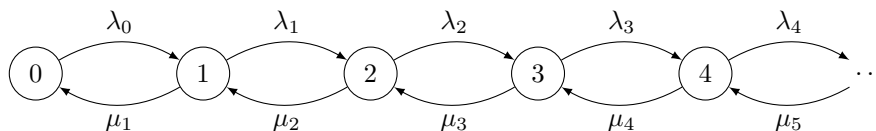
Figure 4.24: A generic Birth-Death Process.
