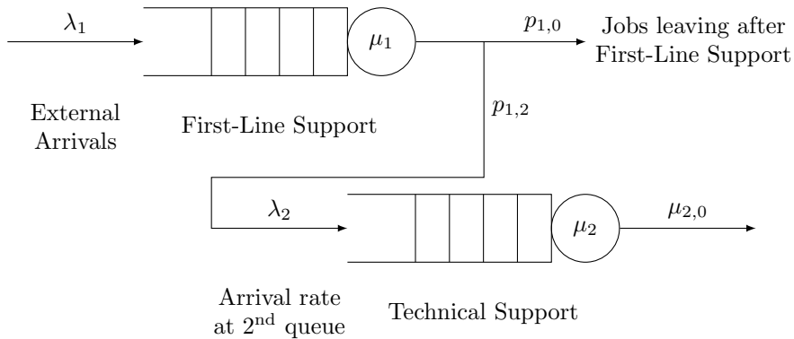
Figure 4.28: A queueing network modeling a two-tier support hotline. Jobs arrive from the outside with rate \lambda_1 and enter the queue for first-line support. After the first-line support served the job, with rate \mu_1 , a p_{1,0} = (1 - p_{1,2}) fraction of the jobs are satisfied and leave the system. The remaining p_{1,2} fraction of jobs need in-depth technical assistance, which is provided by a technician in the technical support queue. Technical support takes time exponentially distributed with parameter \mu_2 , and afterwards the job leaves the system.
