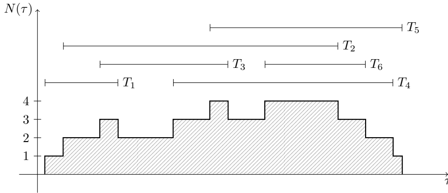
Figure 4.22: A possible realization of the random process describing a queueing system. The jobs and their response times are depicted as segments with lengths T_i , and the number of jobs in the system is given by the curve N(\tau) . In the proof of Little's Law the hatched area is measured in two ways. On the one hand, the hatched area can be obtained by taking the integral of the function N(\tau) . On the other hand, the hatched area is the sum T_1 + \dots + T_6 due to the definition of N(\tau) .
