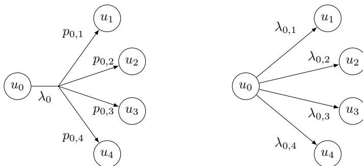
Figure 4.8: Two equivalent views: On the left, the state u_0 has a sojourn time Y exponentially distributed with parameter \lambda_0 . After time Y has passed, the next state is chosen according to the probability distribution (p_{0,1}, p_{0,2}, p_{0,3}, p_{0,4}) . On the right, the sojourn time in state 0 is \min\{Y_1, Y_2, Y_3, Y_4\} , where Y_i \sim \exp(\lambda_{0,i}) with parameter \lambda_{0,i} = p_{0,i} \cdot \lambda_0 . The next state is determined by the random variable that realizes the minimum.
