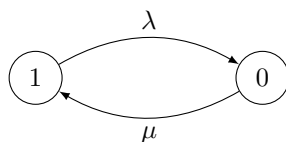
Figure 4.5: A CTMC modeling an unreliable system. In state 1 the system is working, in state 0 the system is faulty. The failure rate , i.e., the time until the system fails, is exponentially distributed with parameter \lambda . After a failure, the repair takes some time, exponentially distributed with parameter \mu .
