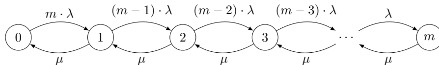
Figure 4.27: Birth-Death process modeling an M/M/1/m/m queueing system.
