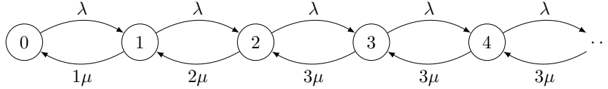
Figure 4.25: Birth-Death process modeling an M/M/3 queueing system. If there are less than 3 jobs, then the number of active servers is the number of jobs in the system. When 3 or more jobs are in the system all servers are active.
