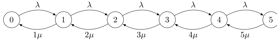
Figure 4.26: Birth-Death process modeling an M/M/5/5 queueing system.
