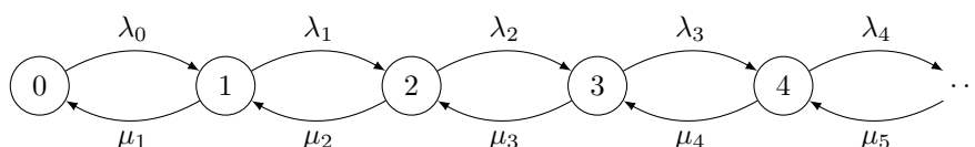
Figure 4.24: A generic Birth-Death Process.
