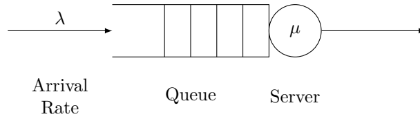
Figure 4.14: A queueing system with one server. Jobs arrive at the queue from a Poisson process with rate \lambda , i.e., the inter-arrival time between two jobs is exponentially distributed with parameter \lambda . If the system is empty, the job is processed immediately, otherwise the job waits in the queue. The time it takes to process a single job is exponentially distributed with parameter \mu , and after one job has been served, if there is a job waiting, the server starts to process the next job.
