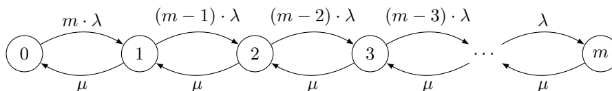
Figure 5.27: Birth-Death process modeling an M/M/1/m/m queueing system.
