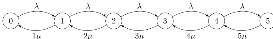
Figure 5.26: Birth-Death process modeling an M/M/5/5 queueing system.
