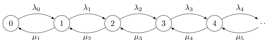
Figure 5.24: A generic Birth-Death Process.
