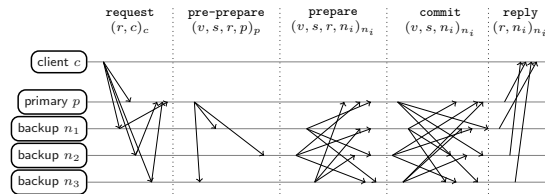
Figure 25.9: The agreement protocol used in PBFT for processing a client request issued by client c , exemplified for a system with n = 4 nodes. The primary in view v is p = n_0 = v \bmod n .
