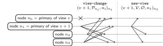
Figure 25.21: The view change protocol used in PBFT. Node n_0 is the primary of current view v , node n_1 the primary of view v + 1 . Once backups consider n_0 to be faulty, they start the view change protocol (cf. Algorithms 25.23, 25.24, 25.25). The X signifies that n_0 is faulty.
