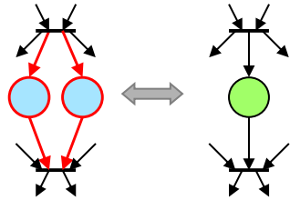
Fusion of Parallel Places (FPP)
