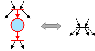
Fusion of Series Transitions (FST)
