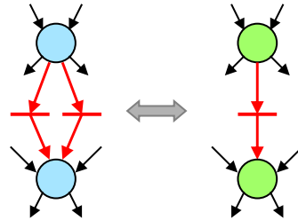
Fusion of Parallel Transitions (FPT)
