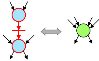
Fusion of Series Places (FSP)
