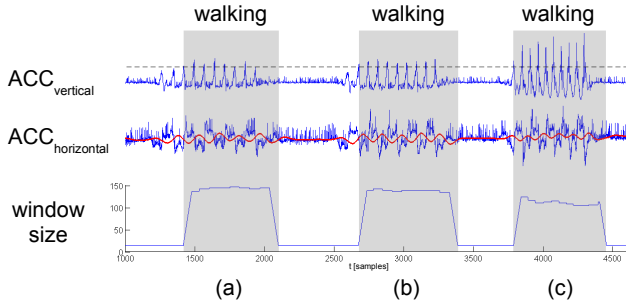
Figure 5. Adaptive filter for artefact compensation while walking slowly (a), moderate (b) and fast (c). Vertical acceleration signal and threshold (dashed line) for detecting walking activity. Horizontal acceleration signal and first derivative for calculating the step length. Resulting window size used by the median filter at the bottom.
