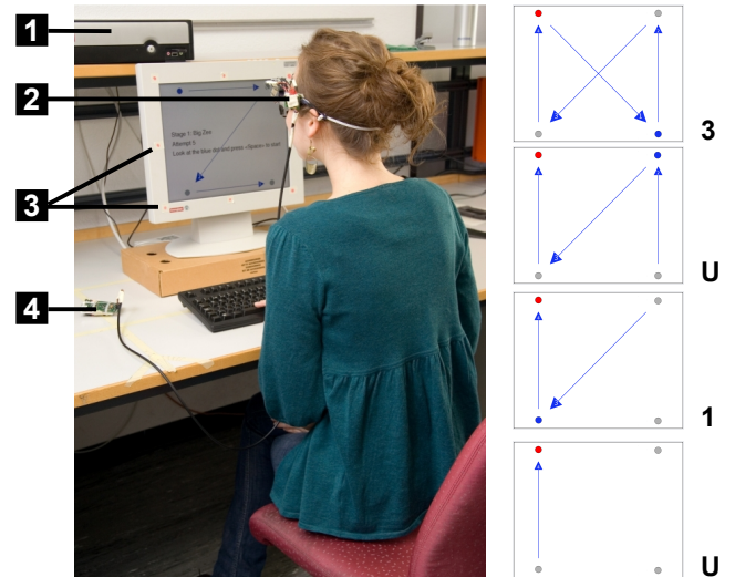
Figure 6. Experimental setup consisting of a desktop computer running the game (1), the Goggles (2), a flat screen with red dots used for calibration (3) and the Pocket (4). The screenshots on the right show the sequence of eye movements and the generated event symbols for gesture 3U1U (from top to bottom). The red dot denotes the start of the gesture and the blue dot its end point. Blue arrows indicate the order and the direction of each expected eye movement and are masked out after having been successfully performed.
