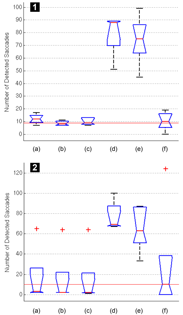
Figure 8. Boxplots for the total number of detected saccades in the horizontal (1) and vertical (2) EOG signal component of run 3 with fixed thresholds T_{saccH} = 700 , T_{saccV} = 2000 over all subjects: stationary/raw (a), stationary/fixed median filter (b), stationary/adaptive filter (c), walking/raw (d), walking/fixed median filter (e), walking/adaptive filter (f). Horizontal red lines in each box indicate the lower quartile, median and upper quartile; dashed vertical lines show the data range; outliers are given as red crosses; the single solid horizontal line indicates the expected number of saccades.
