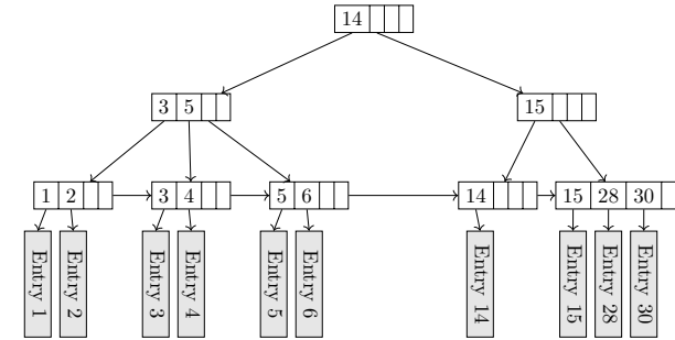
Figure 7.26: Example B+ tree of order b = 4 .
