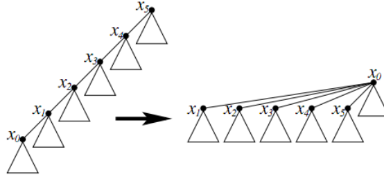
Figure 4.11: Reversal of the path x_0, x_1, x_2, x_3, x_4, x_5 .
