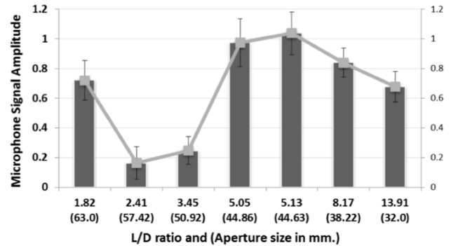
Figure 4: Trend of pressure exerted on a microphone as a function of aperture sizes and associated L/D ratio. Higher amplitude indicates higher relative force. An aperture of 44.63 mm diameter with L/D of 5.13 was selected as optimal.
