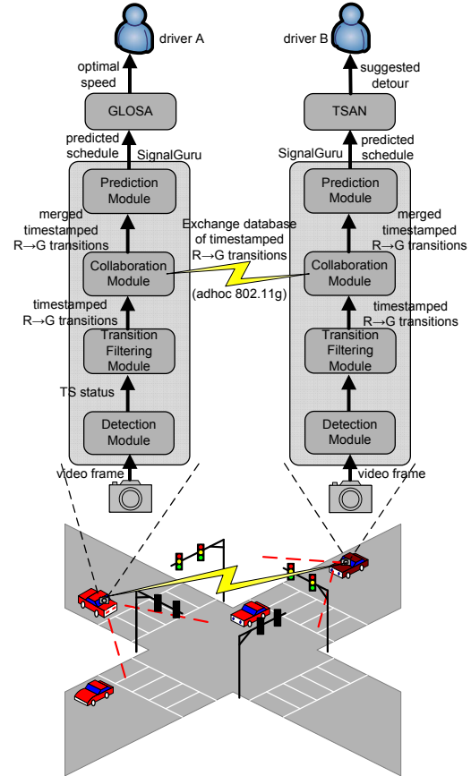
Figure 1: SignalGuru service architecture.
