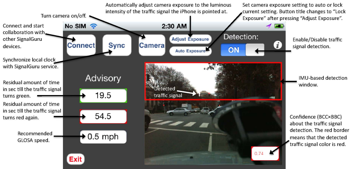
Figure 6: SignalGuru service screenshot. GLOSA advisory has also been included in the same iPhone application. Audio advisory can complement the visual advisory to alleviate driver distraction.
