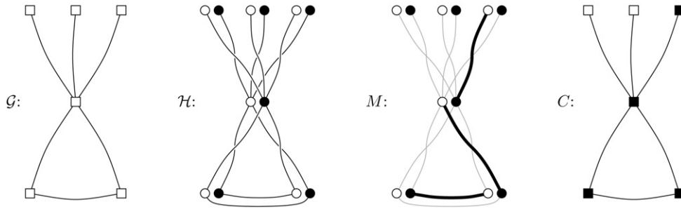
Fig. 1. Algorithm overview.
